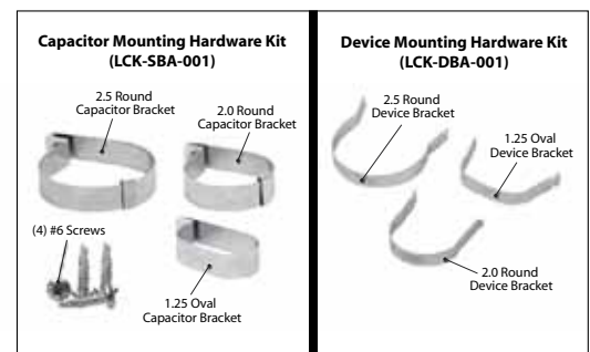
The Life-Line Capacitor Kit also comes with capacitor mounting hardware and self-tapping screws.
