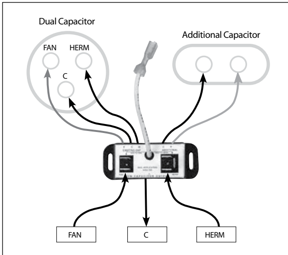
Two Life-Line "Spider" Devices are also included in the kit for use when mounting a combination of capacitors.
