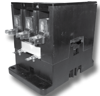
H375AC, H375BC, H375CC, H390AC, H390BC, H390CC Contactors
